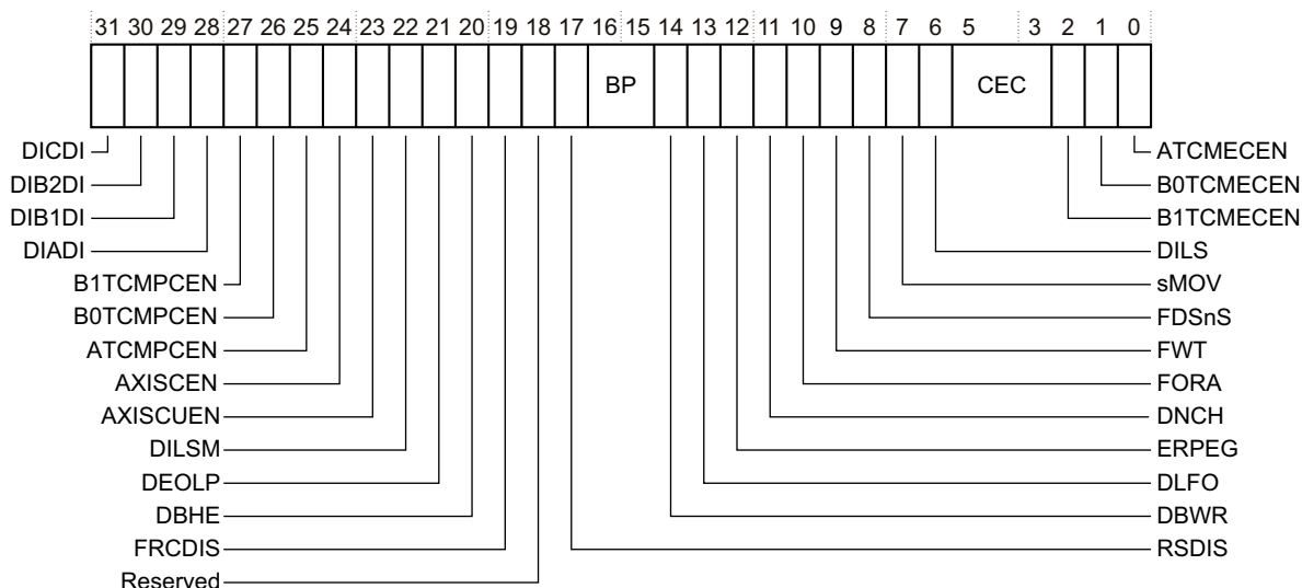
Figure 4-28 ACTLR bit assignments
