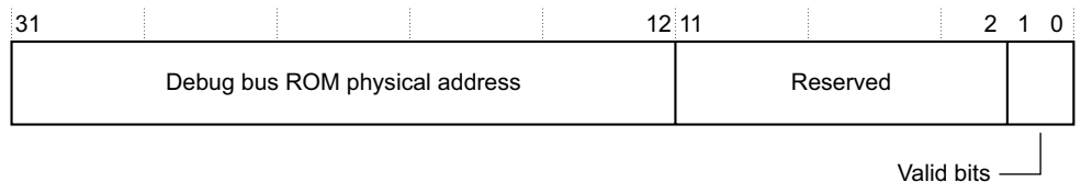
Figure 12-3 DBGDRAR Register bit assignments
