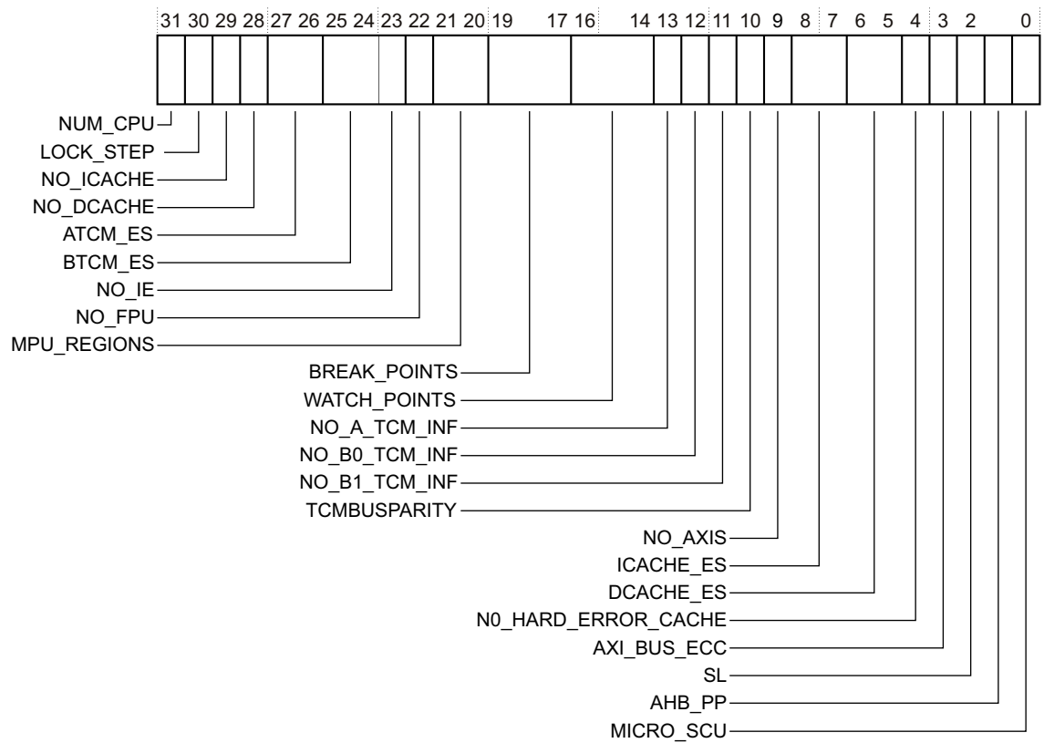
Figure 4-56 Build Options 2 Register bit assignments
