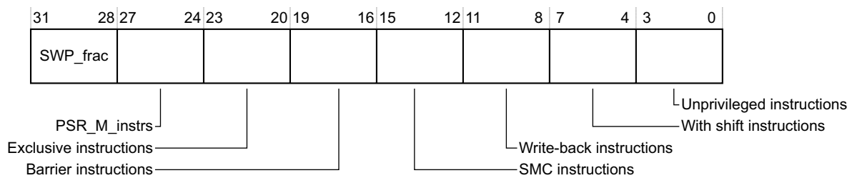
Figure 4-23 ID_ISAR4 bit assignments
