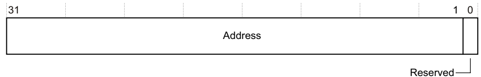
Figure 12-6 DBGWFAR Register bit assignments
