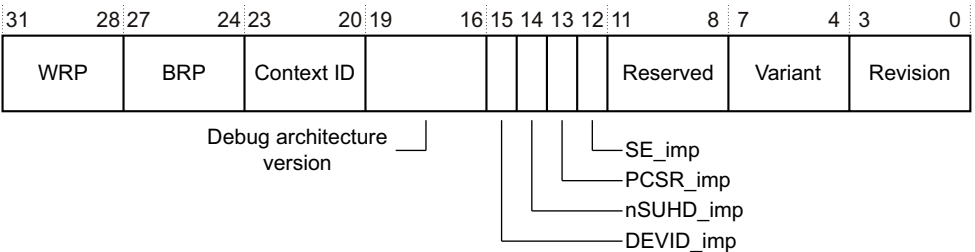
Figure 12-2 DBGDIDR Register bit assignments
