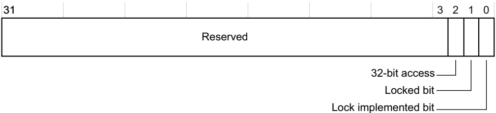
Figure 12-18 DBGLSR Register bit assignments
