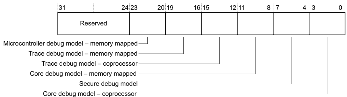
Figure 4-14 ID_DFR0 bit assignments
