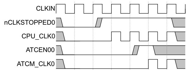
Figure 2-6 Standby, wake-up
