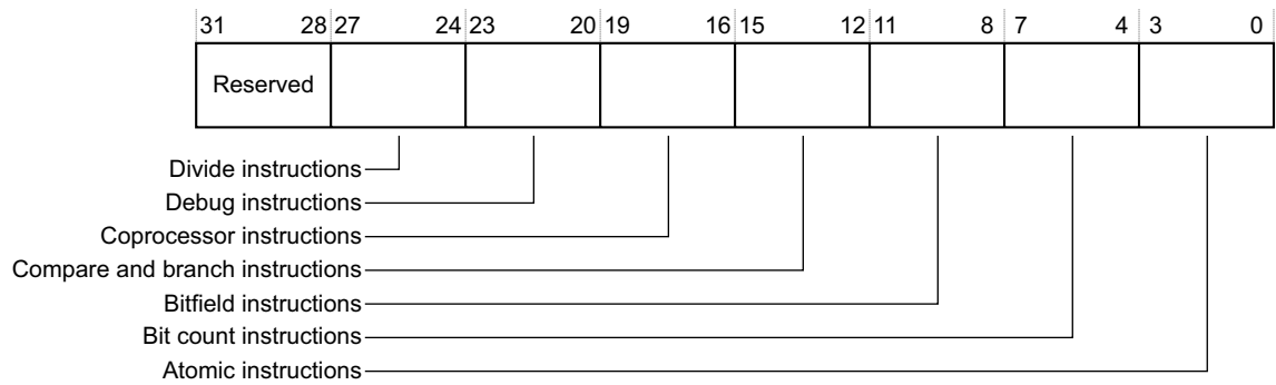
Figure 4-19 ID_ISAR0 bit assignments
