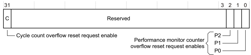
Figure 4-46 nVAL Reset Enable Set Register bit assignments
