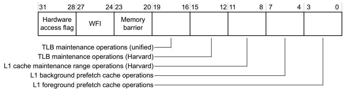
Figure 4-17 ID_MMFR2 bit assignments
