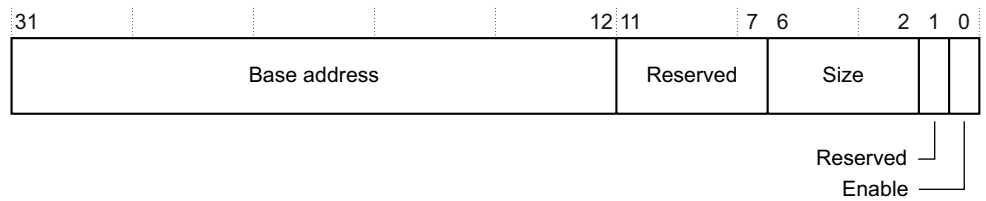
Figure 4-42 ATCM Region Register bit assignments
