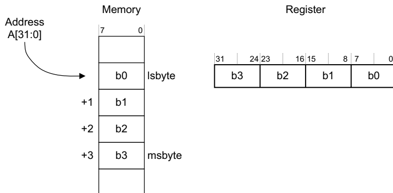
Figure 3-2 Little-endian format
