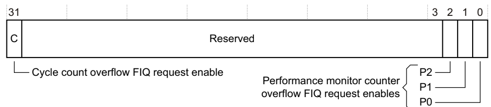
Figure 4-45 nVAL FIQ Enable Set Register bit assignments
