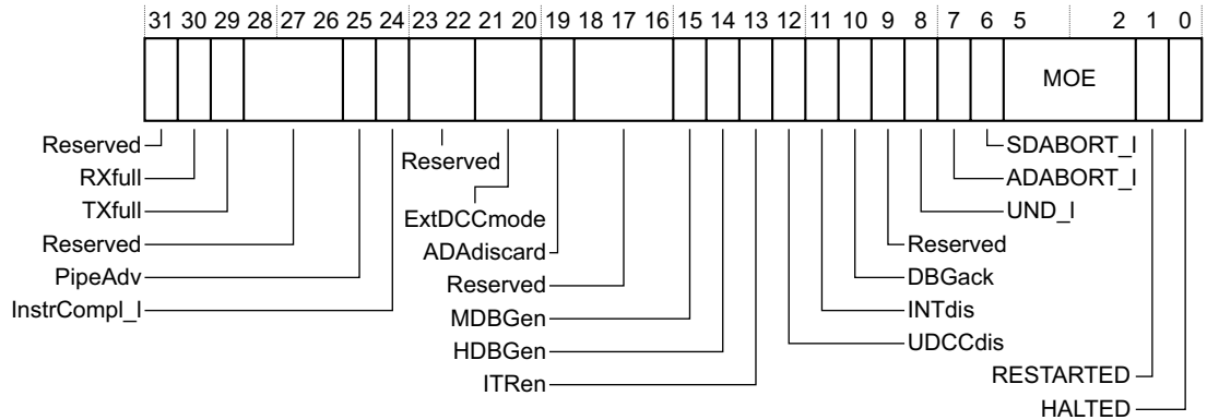
Figure 12-5 DBGDSCR Register bit assignments
