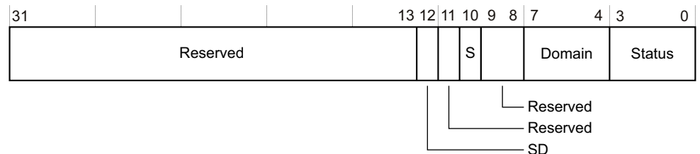
Figure 4-32 IFSR bit assignments
