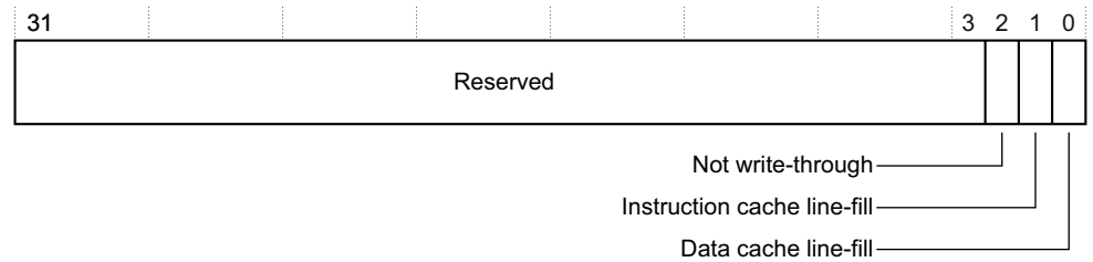
Figure 12-8 DBGDSCCR Register bit assignments
