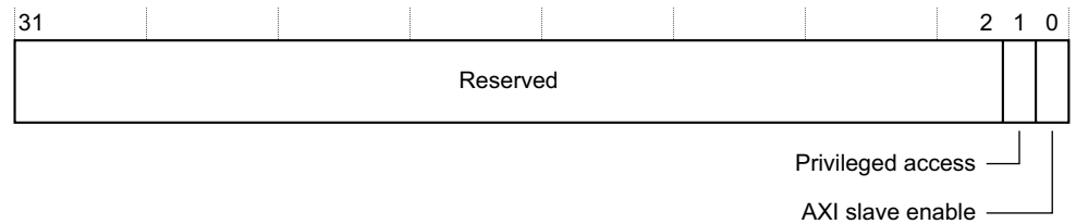
Figure 4-43 Slave Port Control Register bit assignments
