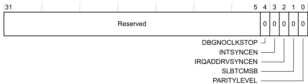
Figure 4-57 Pin Options Register bit assignments
