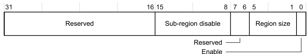
Figure 4-35 MPU Region Size and Enable Registers bit assignments
